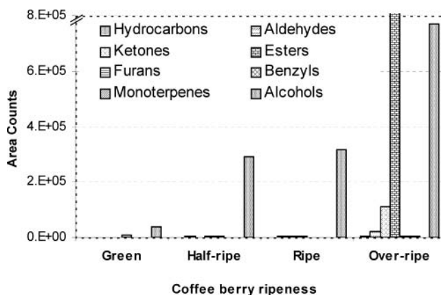
Figure 3. Volatile composition by functional group including the overripe berries to reflect the large intensity of esters and alcohols in this stage of ripeness.
