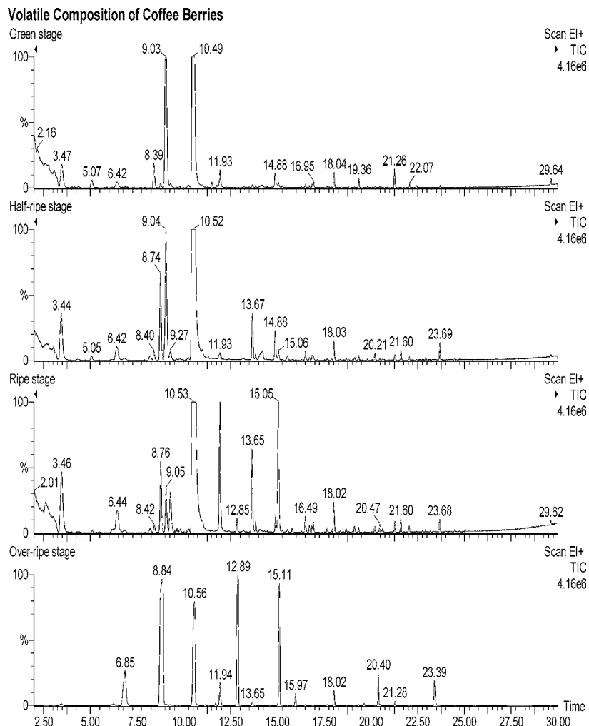
Figure 1. Typical total ion current chromatograms of headspace samples of coffee berries in different stages of ripeness.
