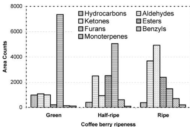
Figure 2. Volatile composition by functional group for green, half-ripe, and ripe berries using data presented in Table 1. Each bar contains the sum of area counts for compounds in each functional group.
